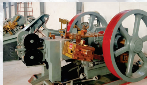
Cold Forging
